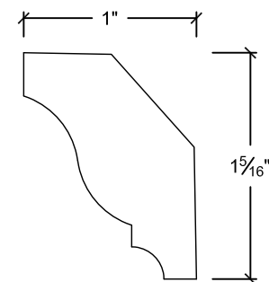
CR1621 5/8" x 1-5/8"
