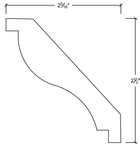
CR3372 3/4" x 3-3/8"
