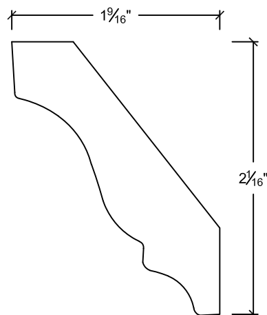
CR2562 5/8" x 2-9/16"
