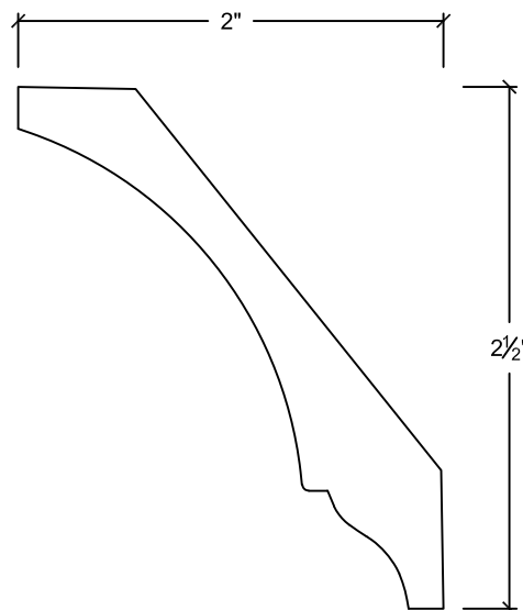
CV3182 9/16" x 3-3/16"
