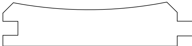
PA3256 3/4" x 3-1/2"
