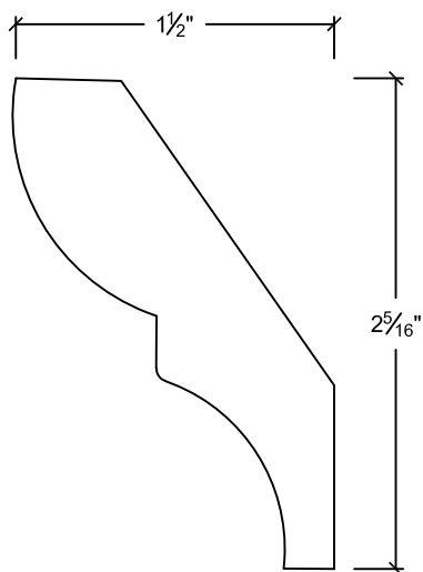
CR2753 11/16" x 2-3/4"
