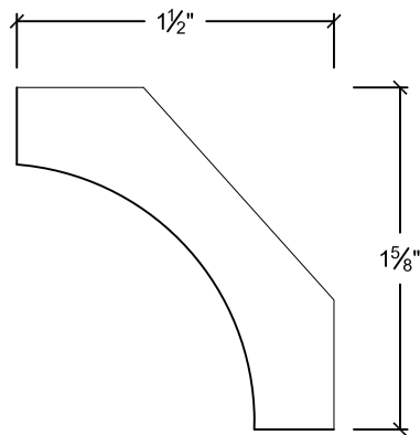
CV2182 11/16" x 2-3/16"
