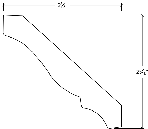
CR3312 9/16" x 3-5/16"
