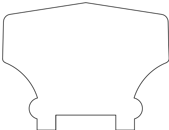
HR2754 2-1/8" x 2-3/4"
