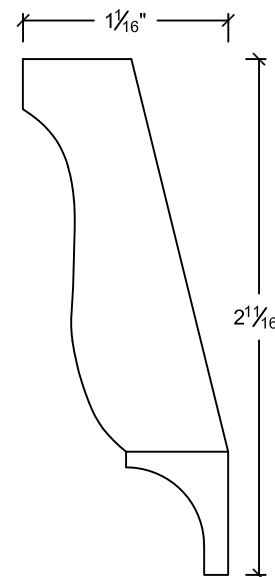
CR2871 (PAIRS WITH CR2812) 11/16" x 2-7/8"
