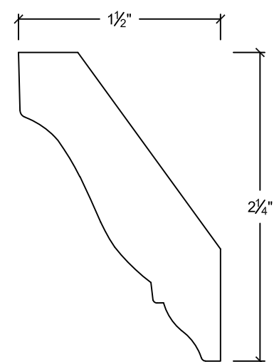
CR2751 5/8" x 2-3/4"
