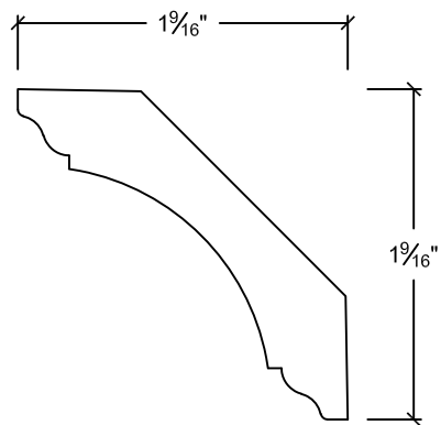
CV2181 1/2" x 2-3/16"
