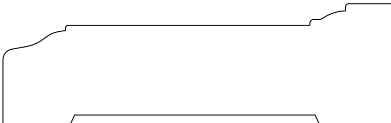
CA4008 1-1/4" x 4"
