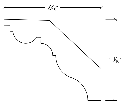
CR2681 3/4" x 2-11/16"
